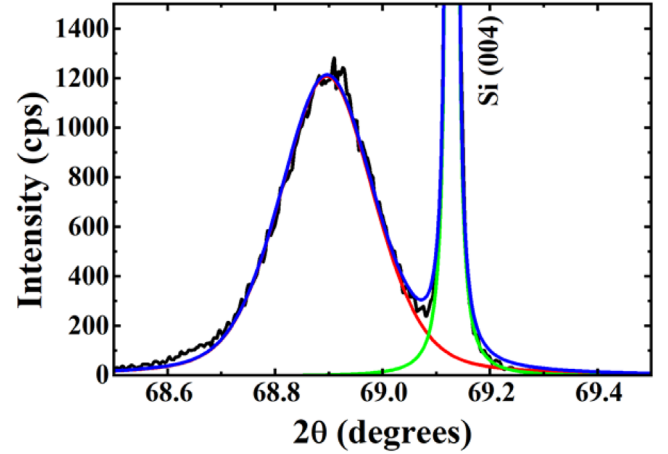
Fig. 2. \theta/2\theta XRD results of the GaP-based n-i-p heterostructure on Si around both the Si (004) and GaP (004) diffraction peaks, and including simulations of the GaP (004) peak (red solid line), the Si (004) peak (green solid line) using a pseudo-Voigt functions. The blue solid line represents the sum of both the simulations.
