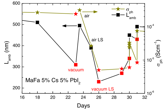
Fig. 8. Evolution of the diffusion length (squares) and of the photoconductivity (stars) of a PVK thin film with its environment (air or vacuum (red symbols)) and with light-soaking. Lines are guides to the eye.
