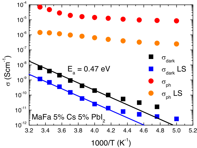
Fig. 4. Arrhenius plots of the dark conductivity (squares) and photoconductivity (circles) of a PVK thin film in its AD and LS states.
