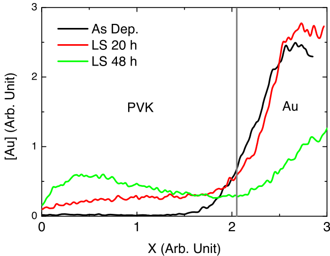
Fig. 11. Gold diffusion through PVK films revealed from GD-OES experiments performed on different films: one in its AD state (black line), LS during 20 h (red line) and 48 h (green line). The vertical grey line indicates the border between the PVK films and the gold electrode.
