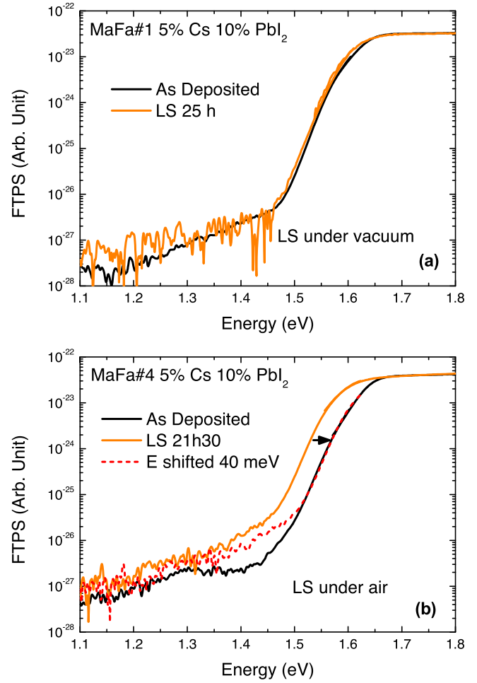
Fig. 10. Evolution of the FTPS spectra of perovskite samples with light-soaking (a) under vacuum, (b) under air, the arrow indicates a shift of 40 meV upward of the LS spectrum.
