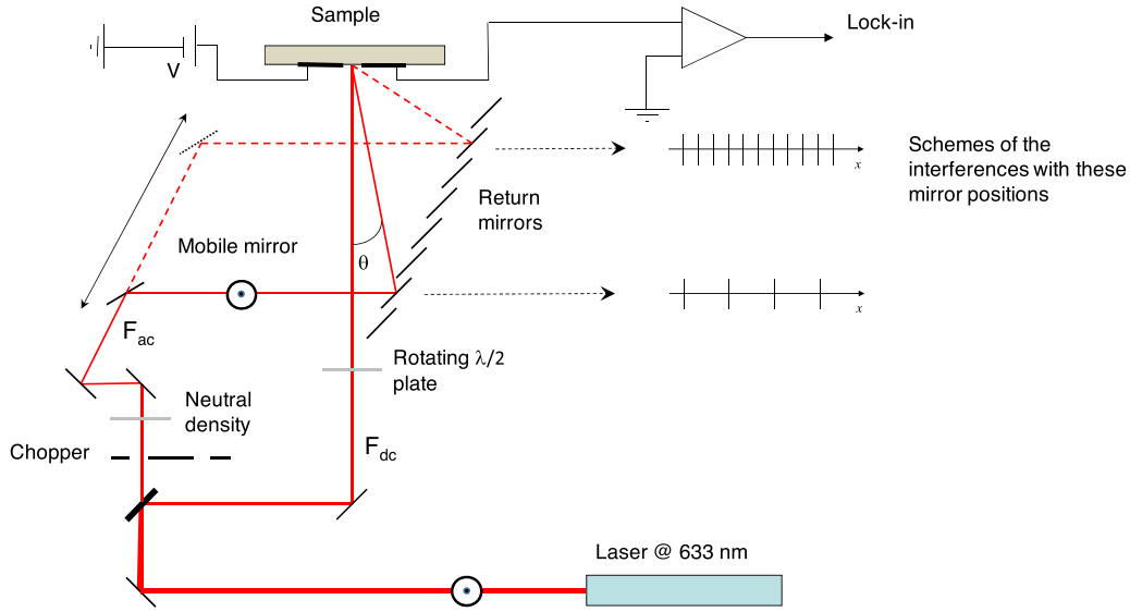
Fig. 1. Schematic diagram of an automatic SSPG bench.
