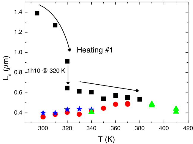
Fig. 6. L_{amb} evolution with several annealings. Black squares correspond to the first annealing up to 380 K (arrows indicate the L_{amb} evolution). Blue stars correspond to the L_{amb} evolution after this annealing. Red circles give the L_{amb} evolution after a second annealing at 370 K during 1h10 and the green triangles were obtained after subsequent annealings at 390 and 410 K.
