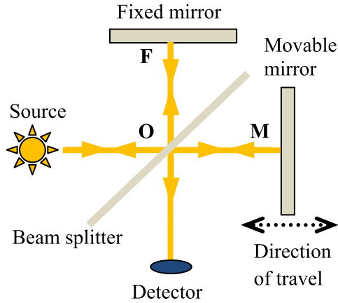
Fig. 2. Schematic diagram of a Michelson interferometer.
