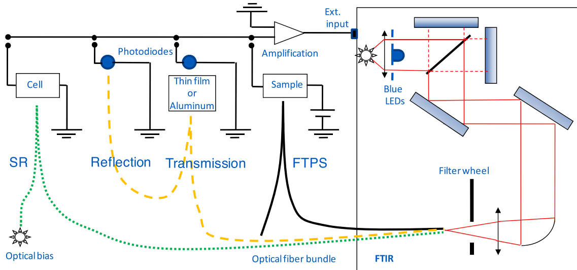
Fig. 3. Schematic diagram of a versatile FTSP set-up.
