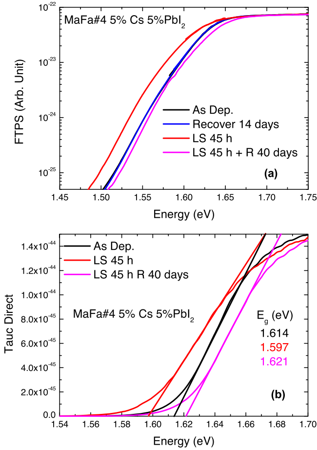
Fig. 9. Evolution with time and light-soaking, (a) of the FTPS spectra, (b) of the Tauc gap of a perovskite thin film.
