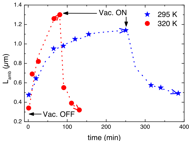
Fig. 7. Evolution of the diffusion lengths measured when the sample is put under air (vac. OFF) or under vacuum (vac. ON) at two temperatures: 295 K (stars), 320 K (circles). Dashed arrows are guides to the eye.
